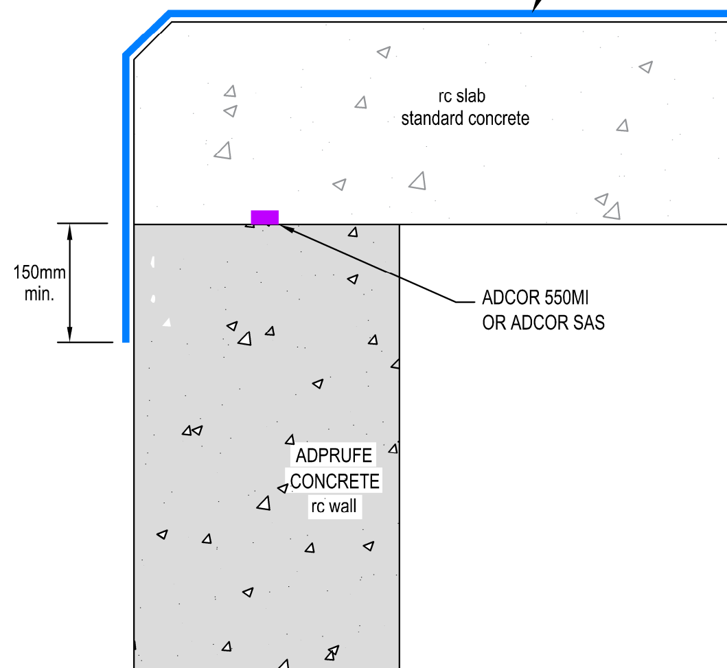
SECTION BETWEEN CONSTRUCTION JOINTS
