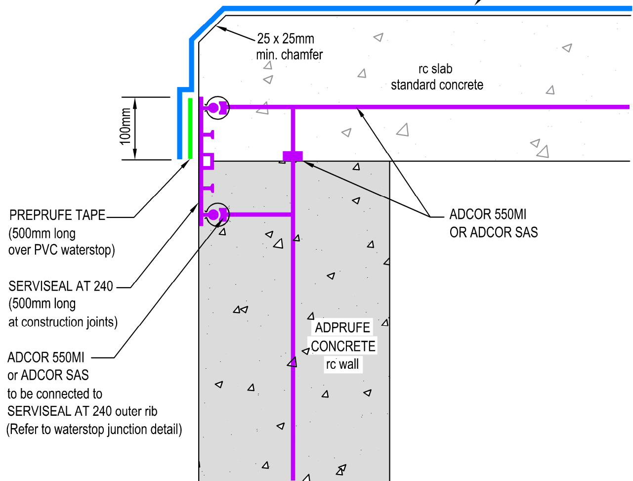
SECTION AT CONSTRUCTION JOINT
