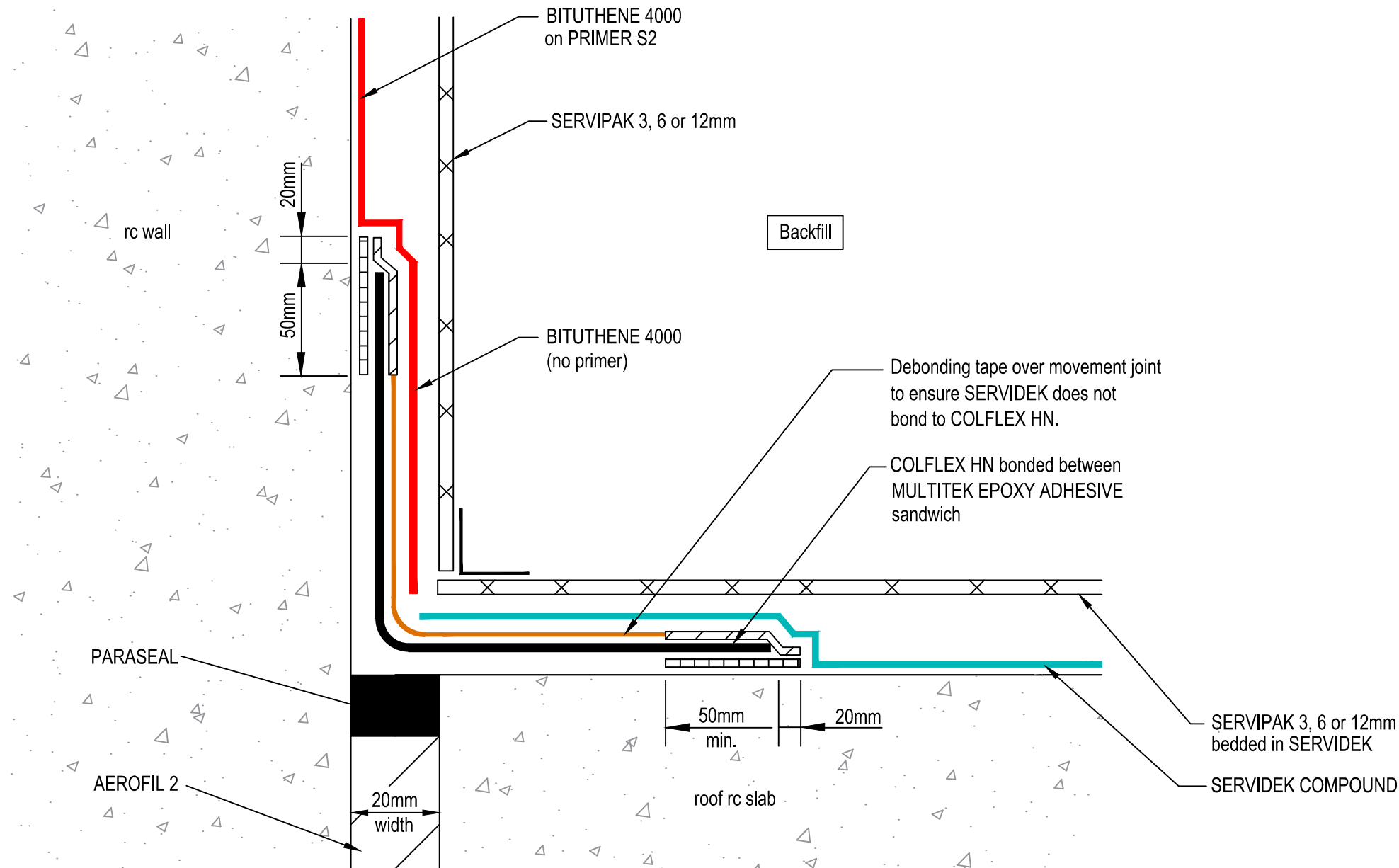
BURIED DECK MOVEMENT JOINT - COLFLEX HN MAXIMUM ELONGATION = 20MM SECTION
