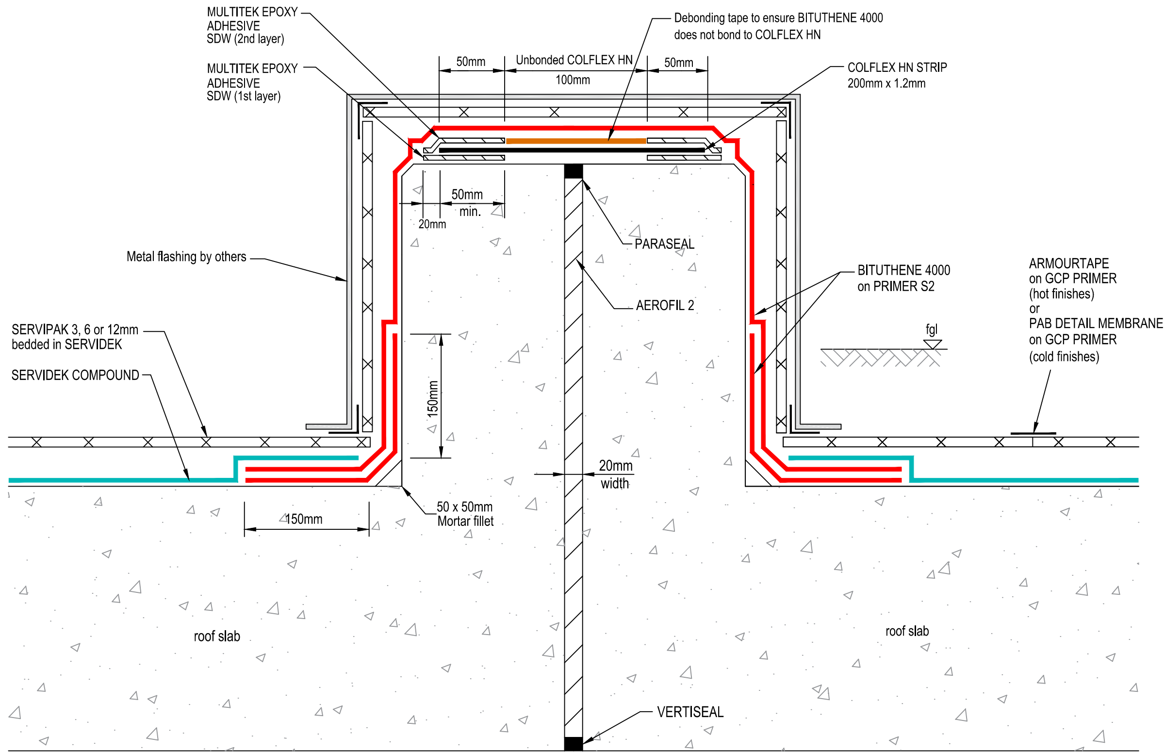
MOVEMENT JOINT - UPSTAND - COLFLEX HN MAXIMUM ELONGATION = 20MM SECTION
