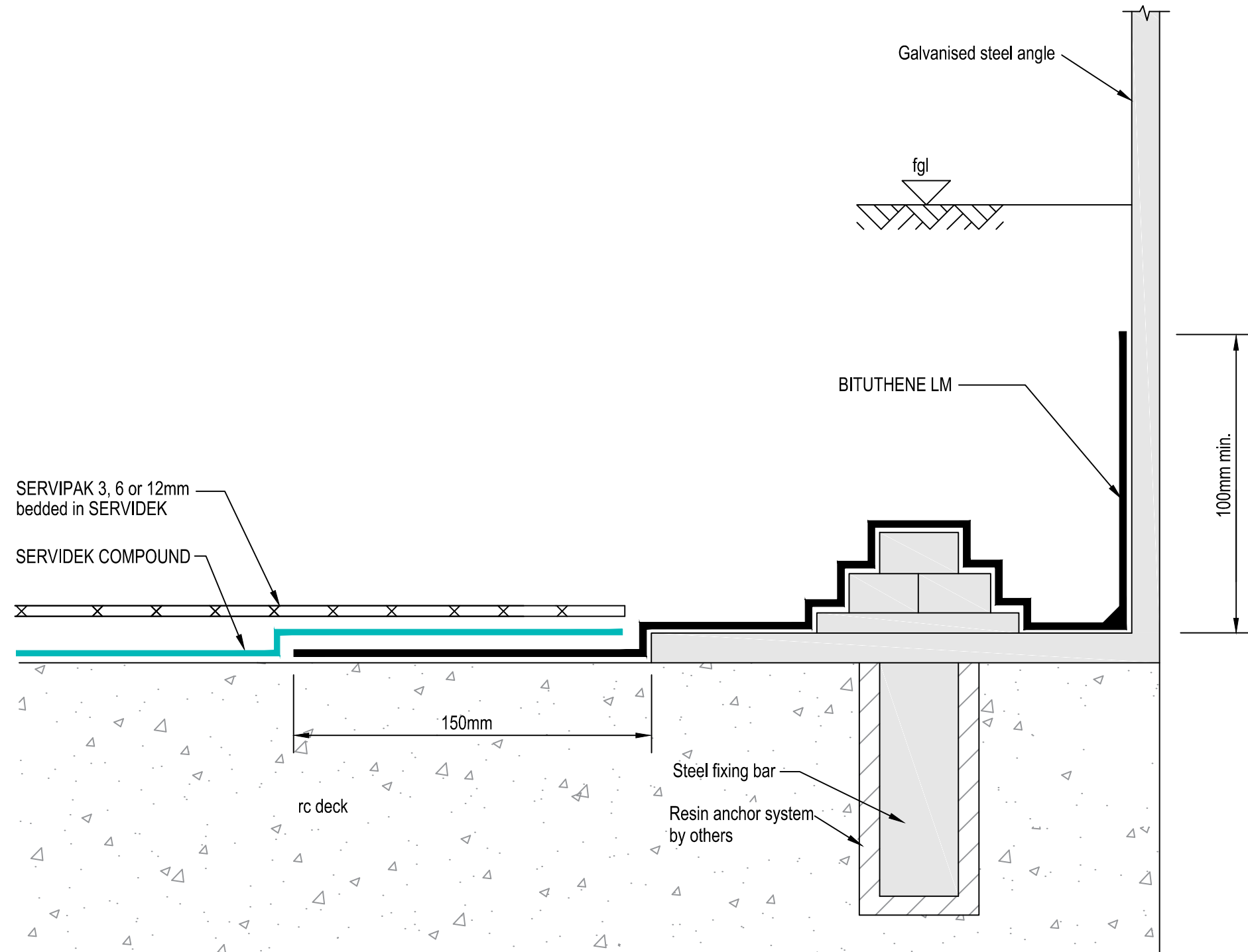
ROOF DECK PERIMETER - METAL UPSTAND - COLD FINISHES SECTION
