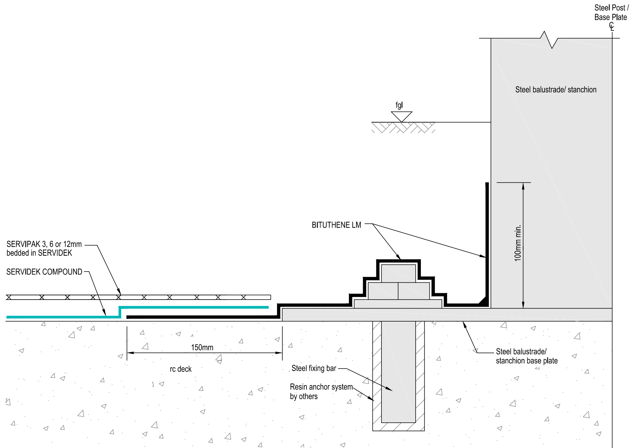
BALUSTRADE POST / STANCHION BASE PLATE - COLD FINISHES SECTION
