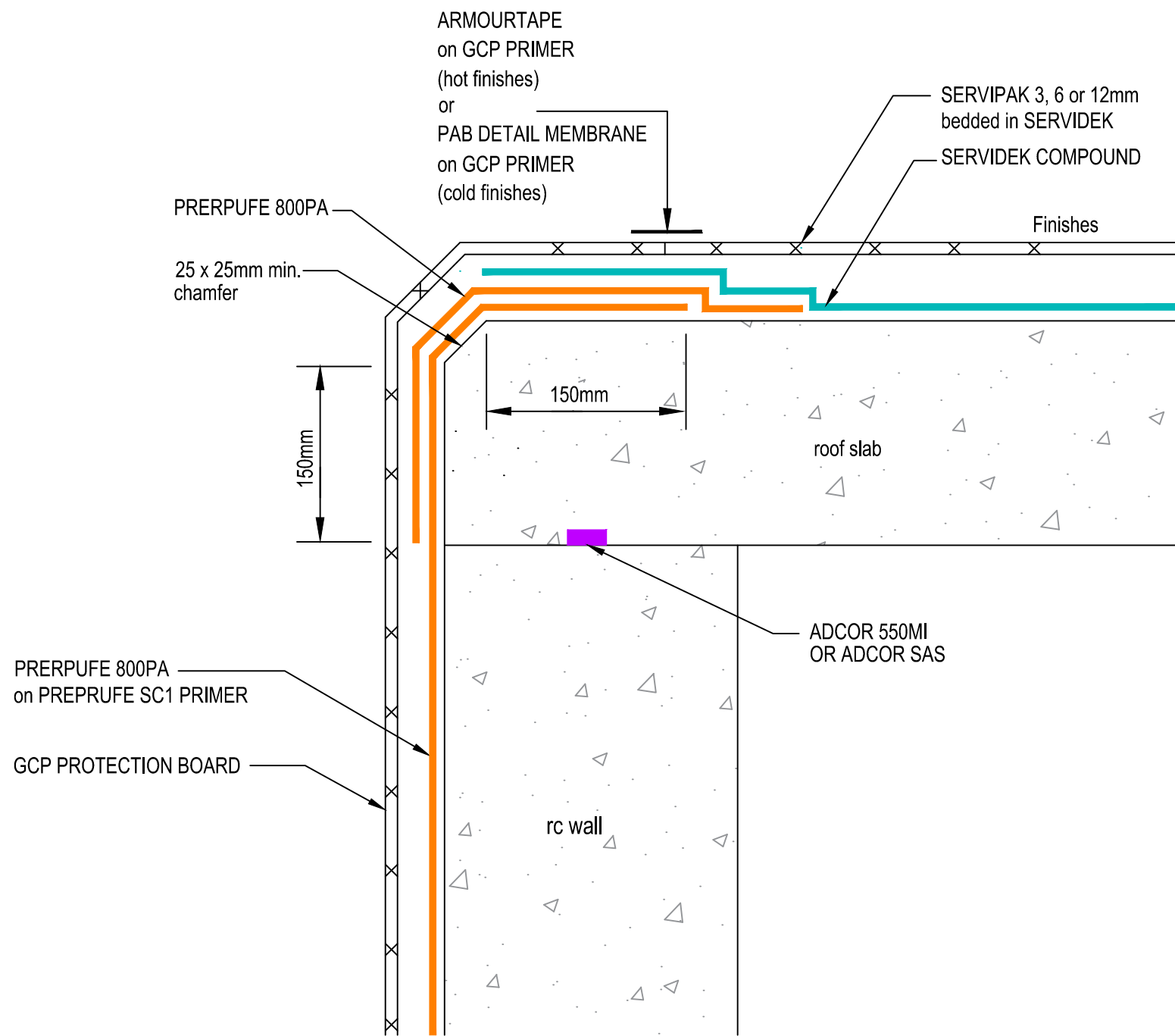
RC WALL / DECK INTERFACE PREPRUFE 800PA / SERVIDEK-SERVIPAK SECTION
