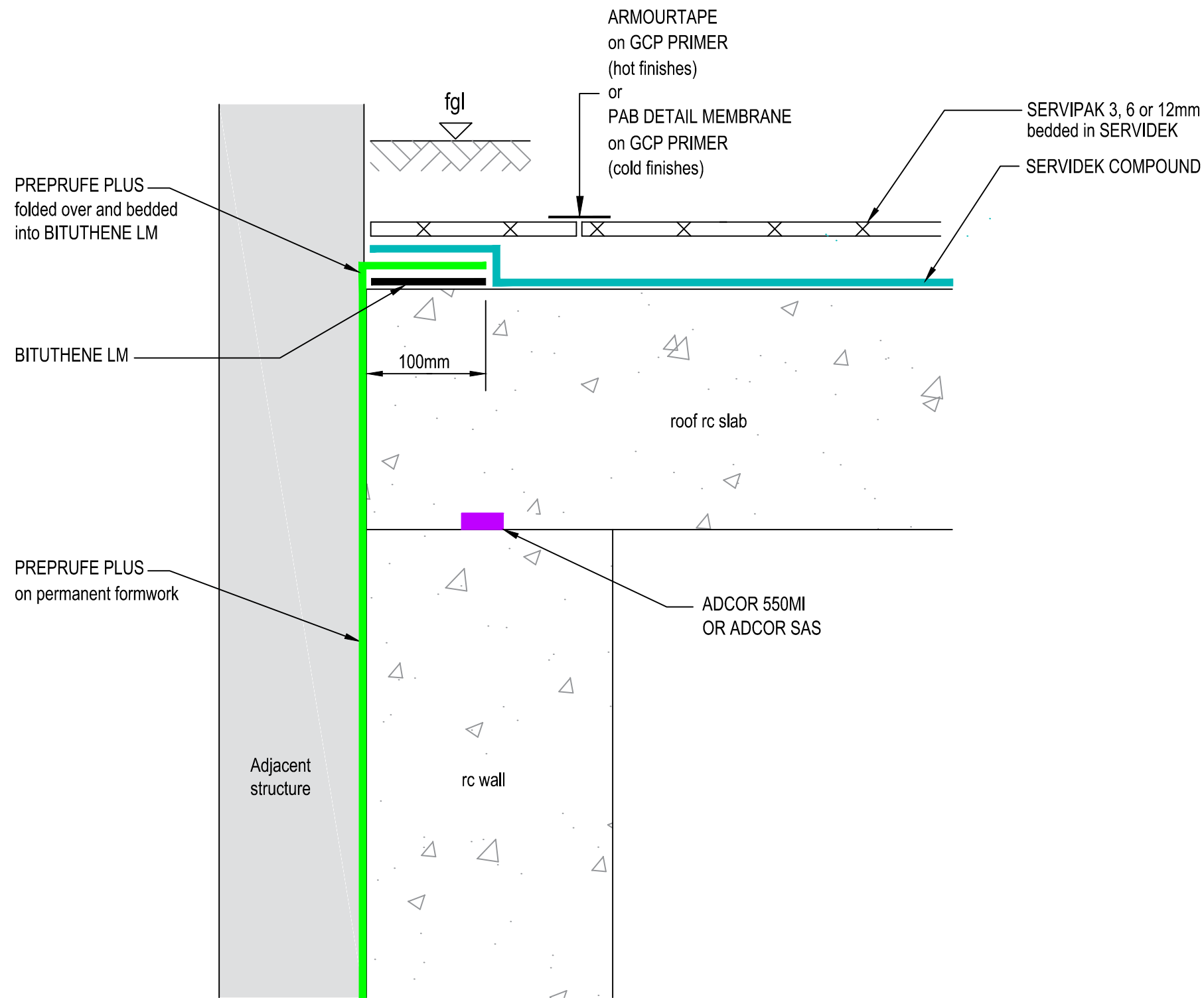
RC WALL / DECK INTERFACE PREPRUFE PLUS / SERVIDEK-SERVIPAK (CONFINED SITE) SECTION
