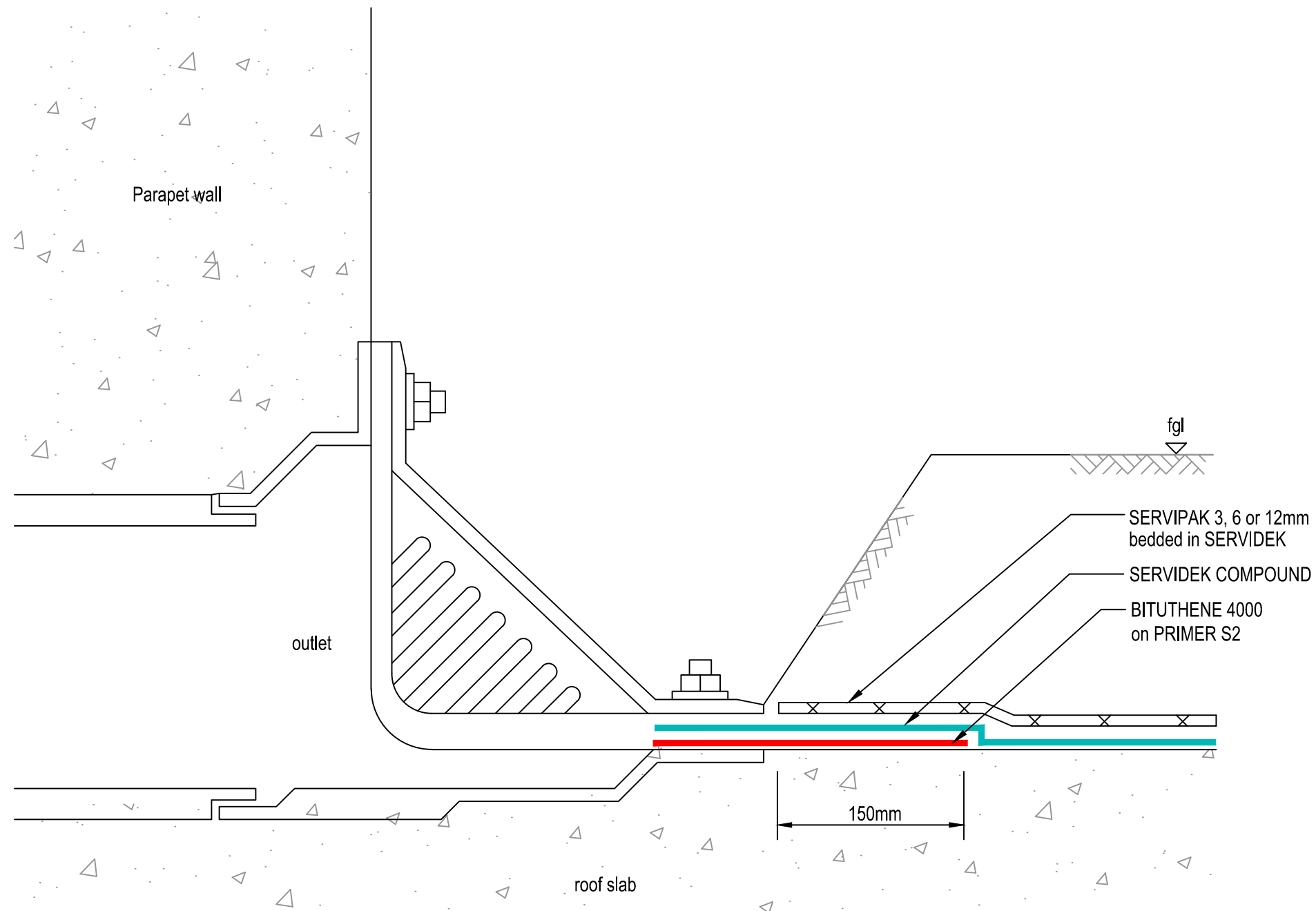
SIDE ENTRY OUTLET SECTION Servidek / Servipak System
