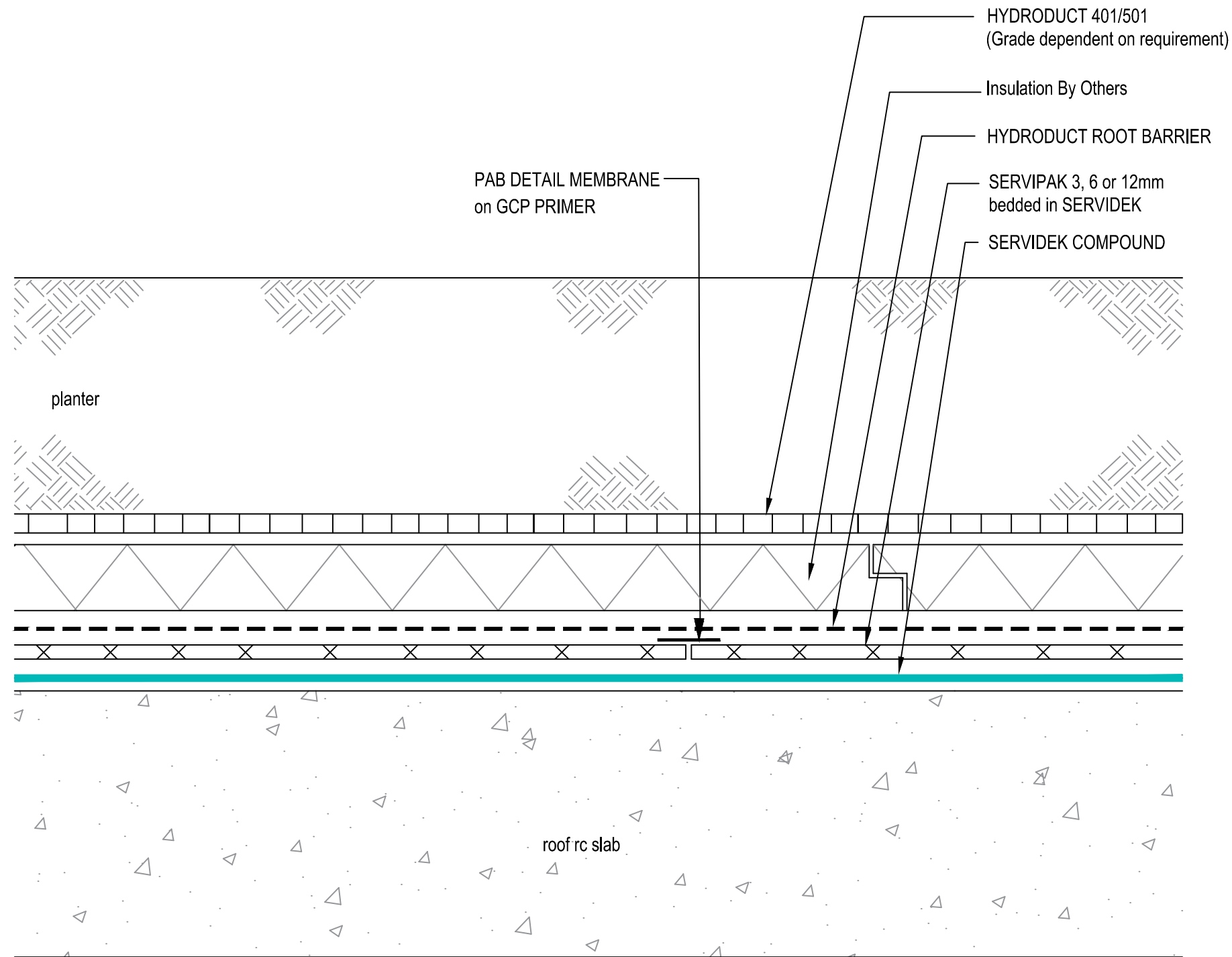
TYPICAL DECK SECTION INSULATED PLANTER Servidek / Servipak System
