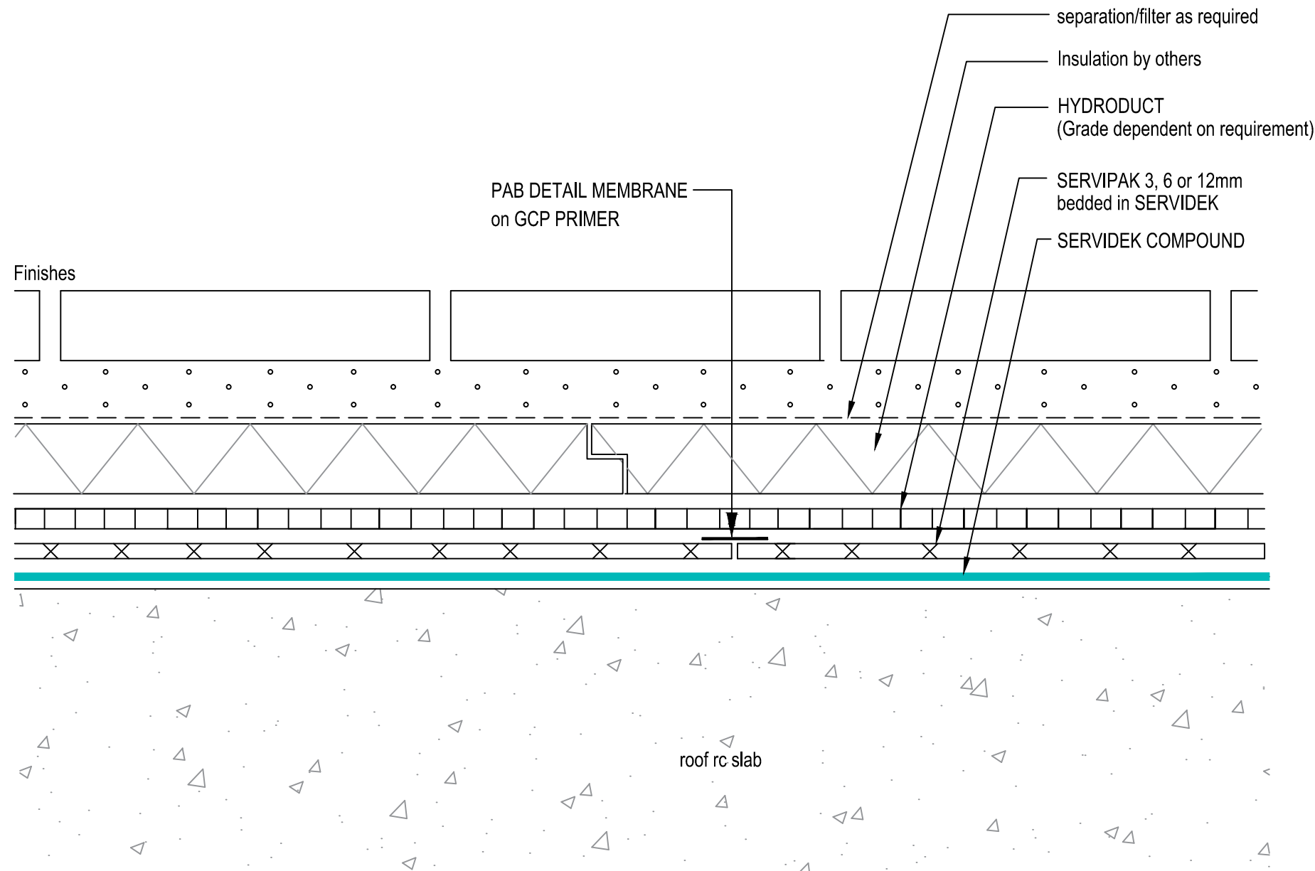
TYPICAL DECK SECTION WITH FINISHES INSULATED / DRAINED Servidek / Servipak System
