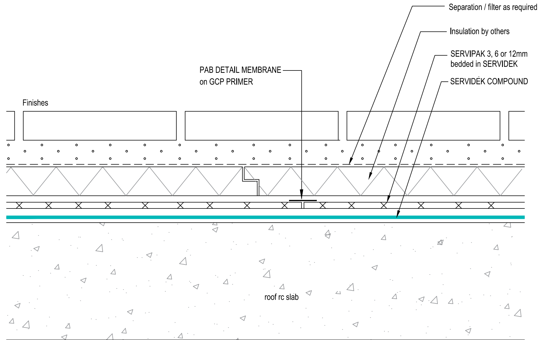
TYPICAL DECK SECTION WITH FINISHES INSULATED Servidek / Servipak System
