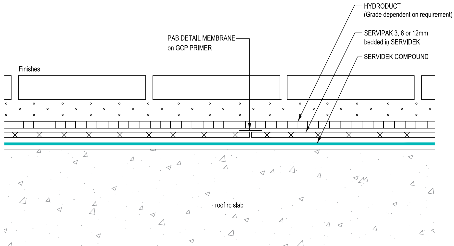
TYPICAL DECK SECTION WITH FINISHES DRAINED Servidek / Servipak System
