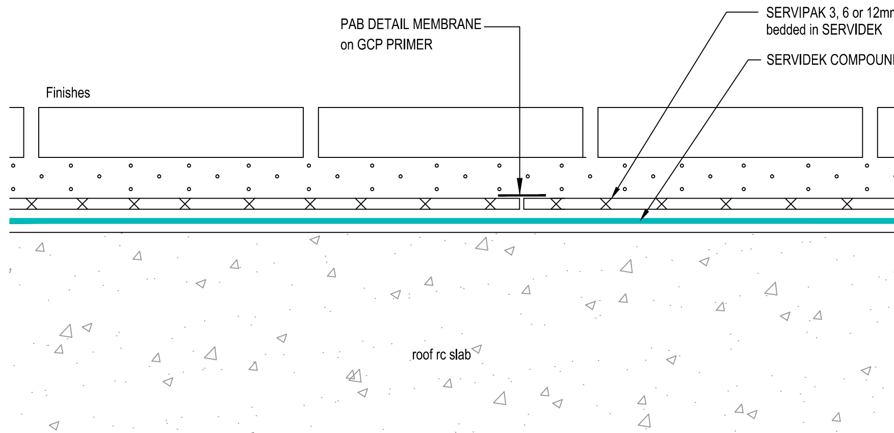
TYPICAL DECK SECTION WITH FINISHES
