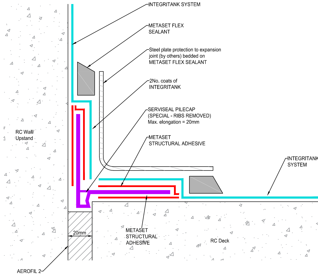
DECK EXPANSION JOINT SERWISEAL PILECAP (SPECIAL - RIBS REMOVED) Max. Elongation = 20 mm Section
