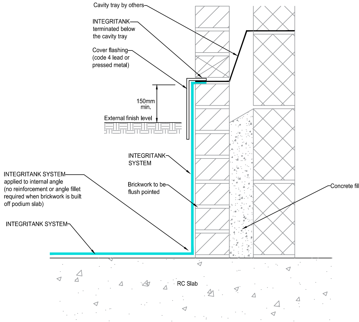
TERMINATION TO OUTER LEAF OF WALL CAVITY Section
