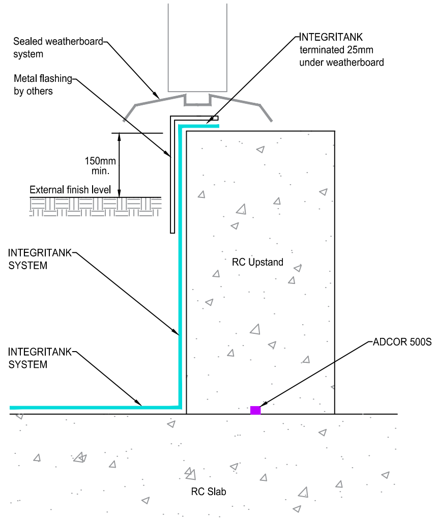
TERMINATION TO RC UPSTAND Section
