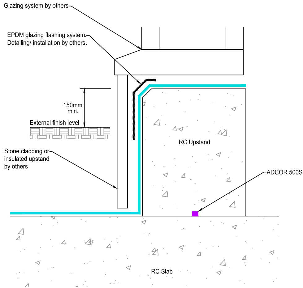
TERMINATION - CLADDING / GLAZING Section
