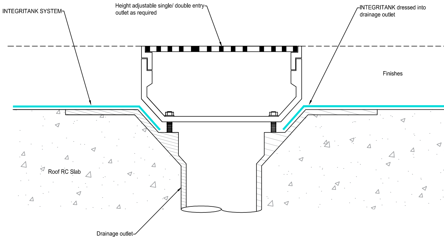
SINGLE / DOUBLE ENTRY OUTLET Section
