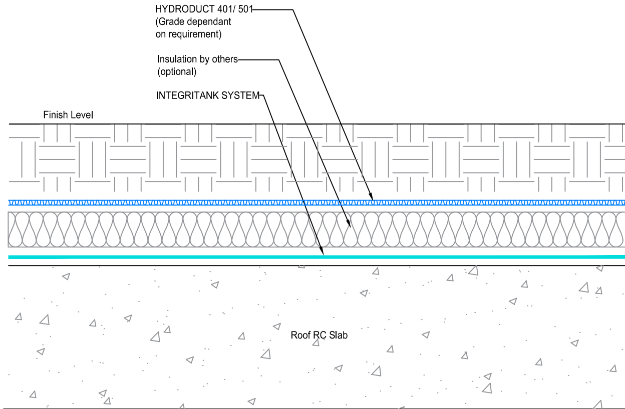
TYPICAL DECK WITH PLANTER FINISHES Section
