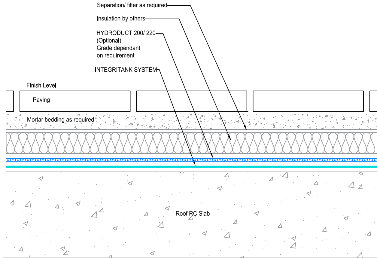
TYPICAL DECK WITH INSULATED FINISHES Section
