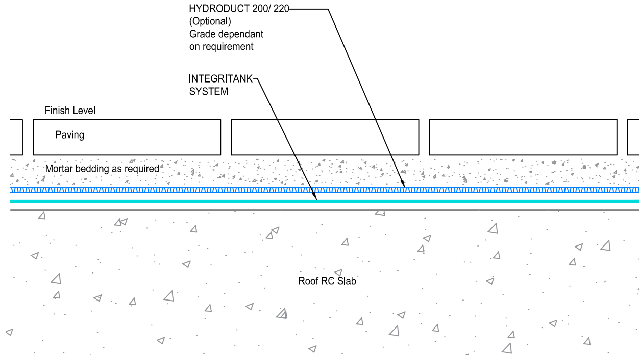
TYPICAL DECK WITH FINISHES Section
