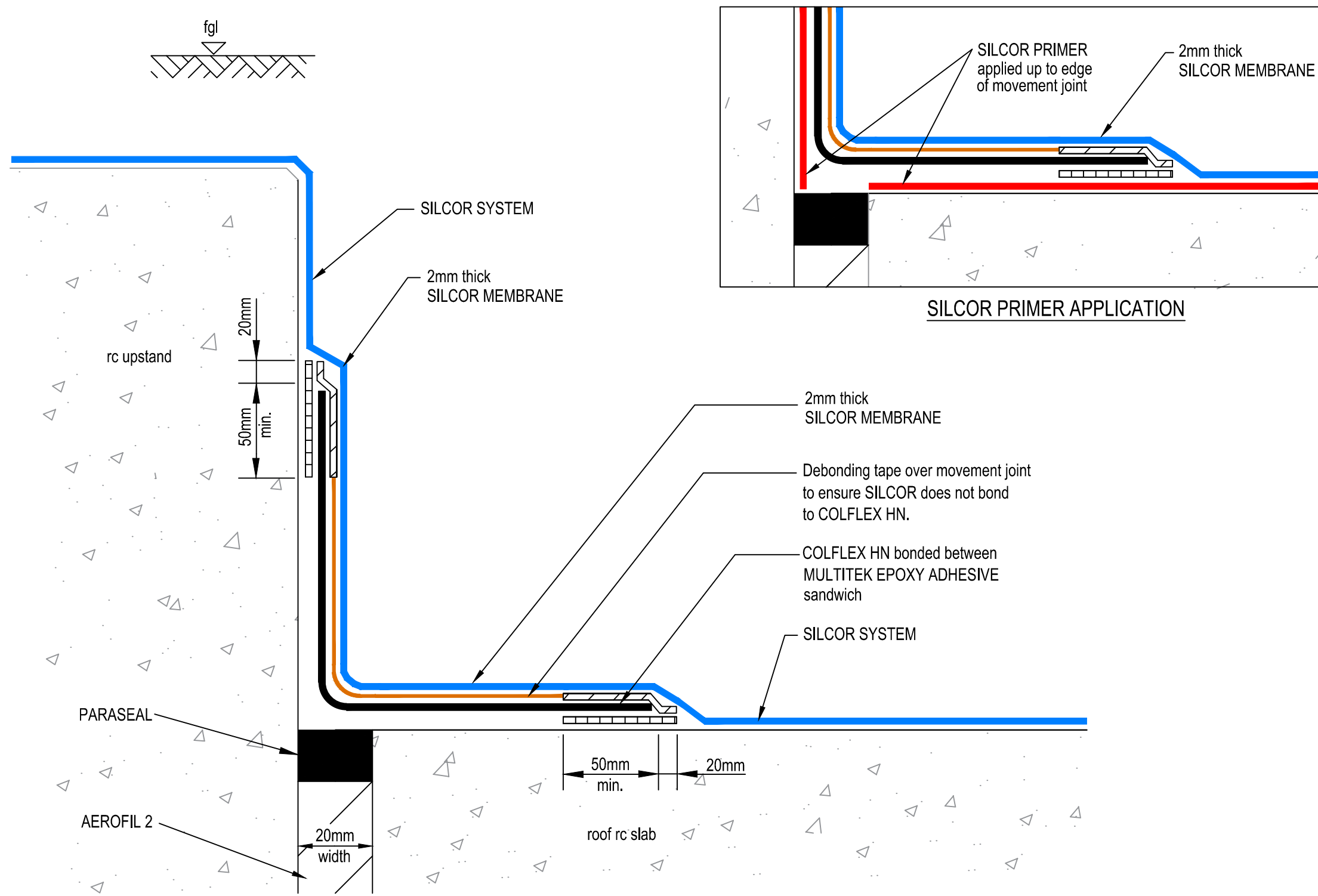
BURIED DECK MOVEMENT JOINT - COLFLEX HN MAXIMUM ELONGATION = 20MM SECTION
