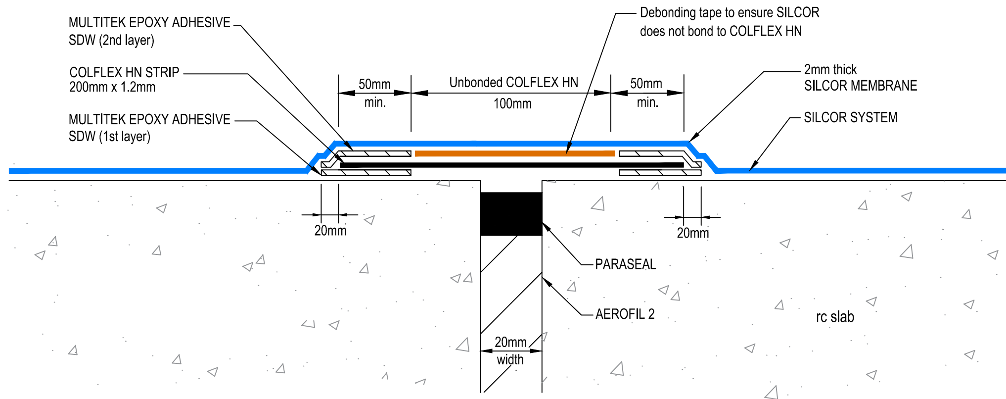
MOVEMENT JOINT - COLFLEX HN MAXIMUM ELONGATION = 20MM SECTION
