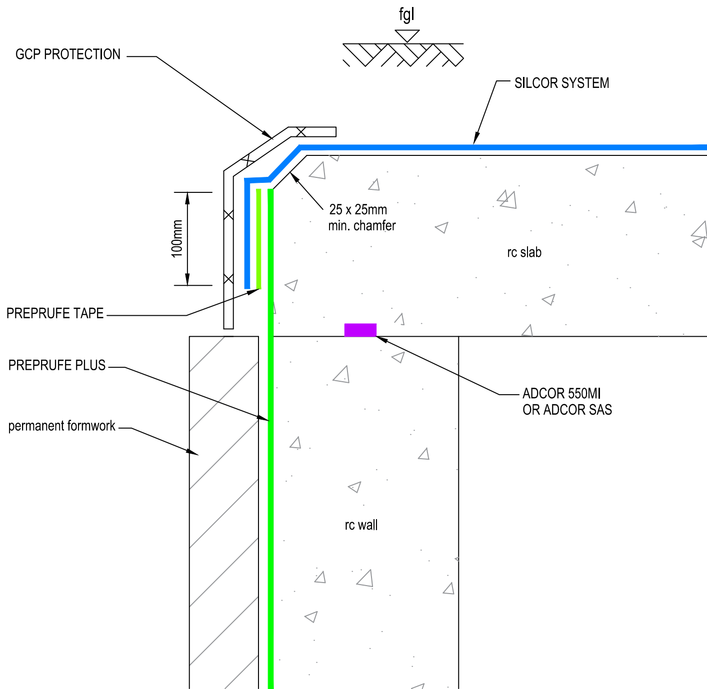
RC WALL / DECK INTERFACE PREPRUFE PLUS / SILCOR SECTION
