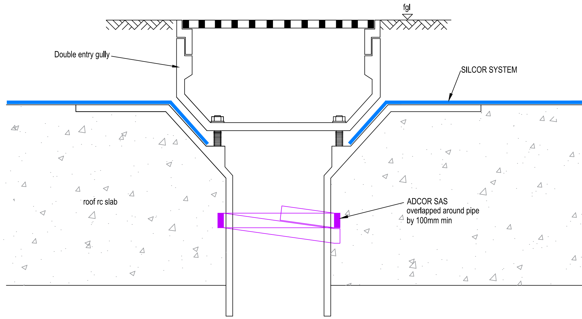
DOUBLE ENTRY OUTLET SECTION
