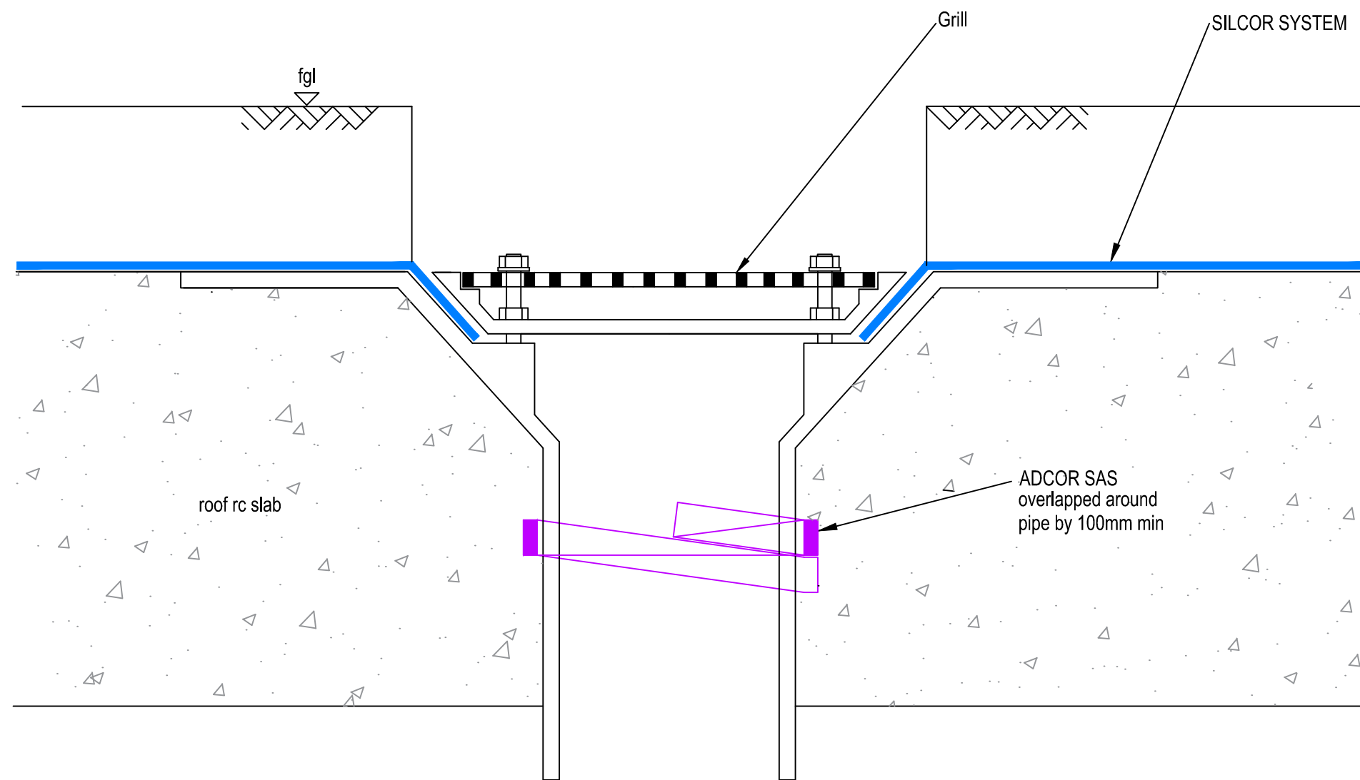
SINGLE ENTRY OUTLET SECTION
