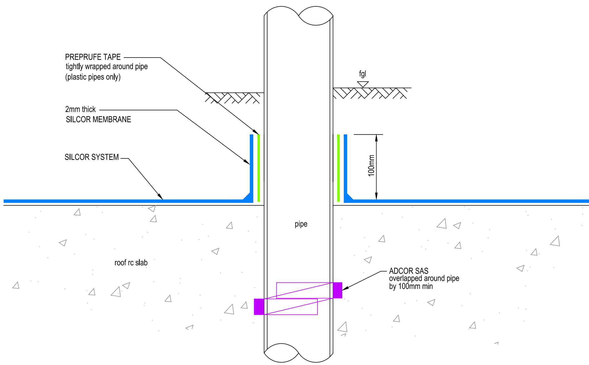
PIPE PENETRATION (PRE-INSTALLED PIPE) SECTION
