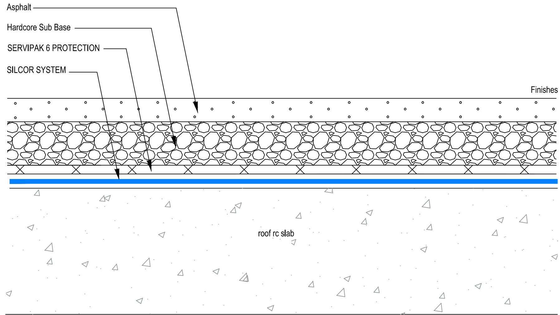
TYPICAL CAR PARK DECK SECTION WITH FINISHES ASPHALT ON HARDCORE SUB-BASE
