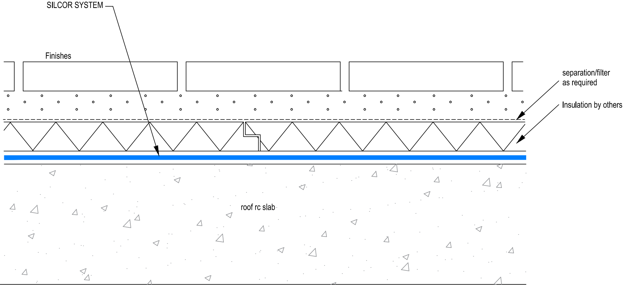
TYPICAL DECK SECTION WITH FINISHES INSULATED
