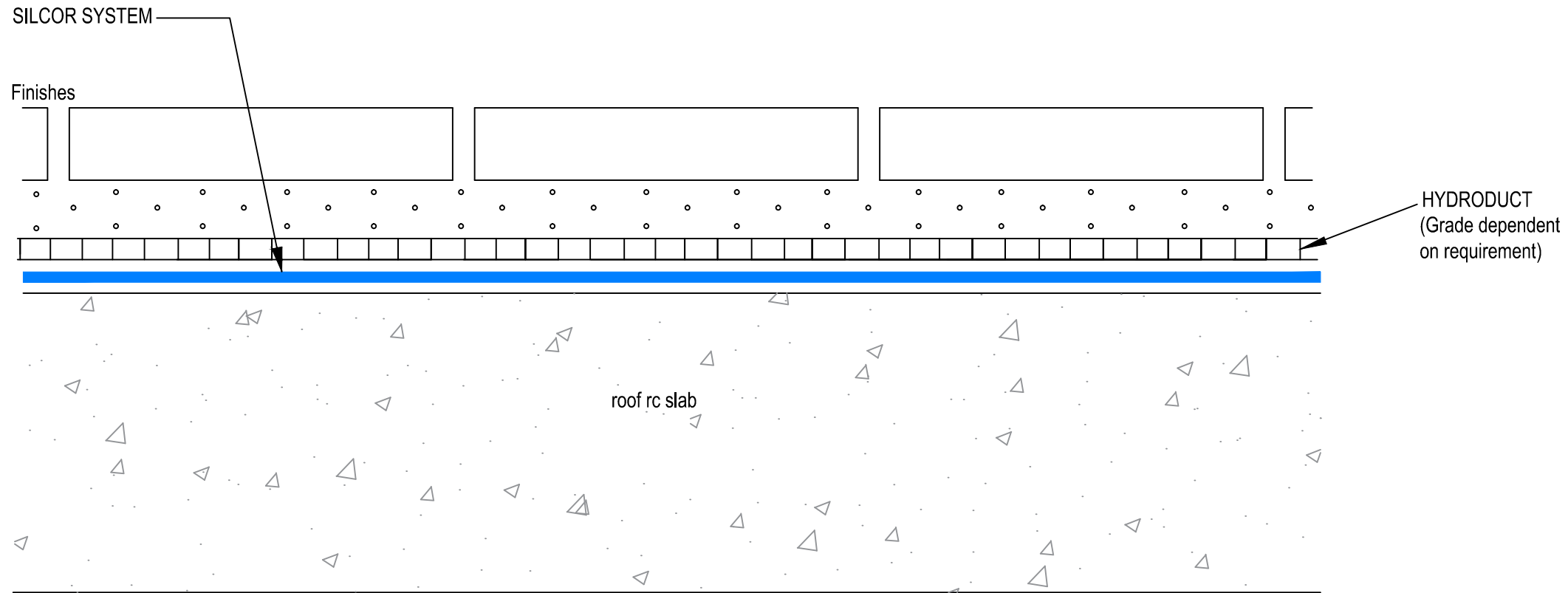
TYPICAL DECK SECTION WITH FINISHES DRAINED
