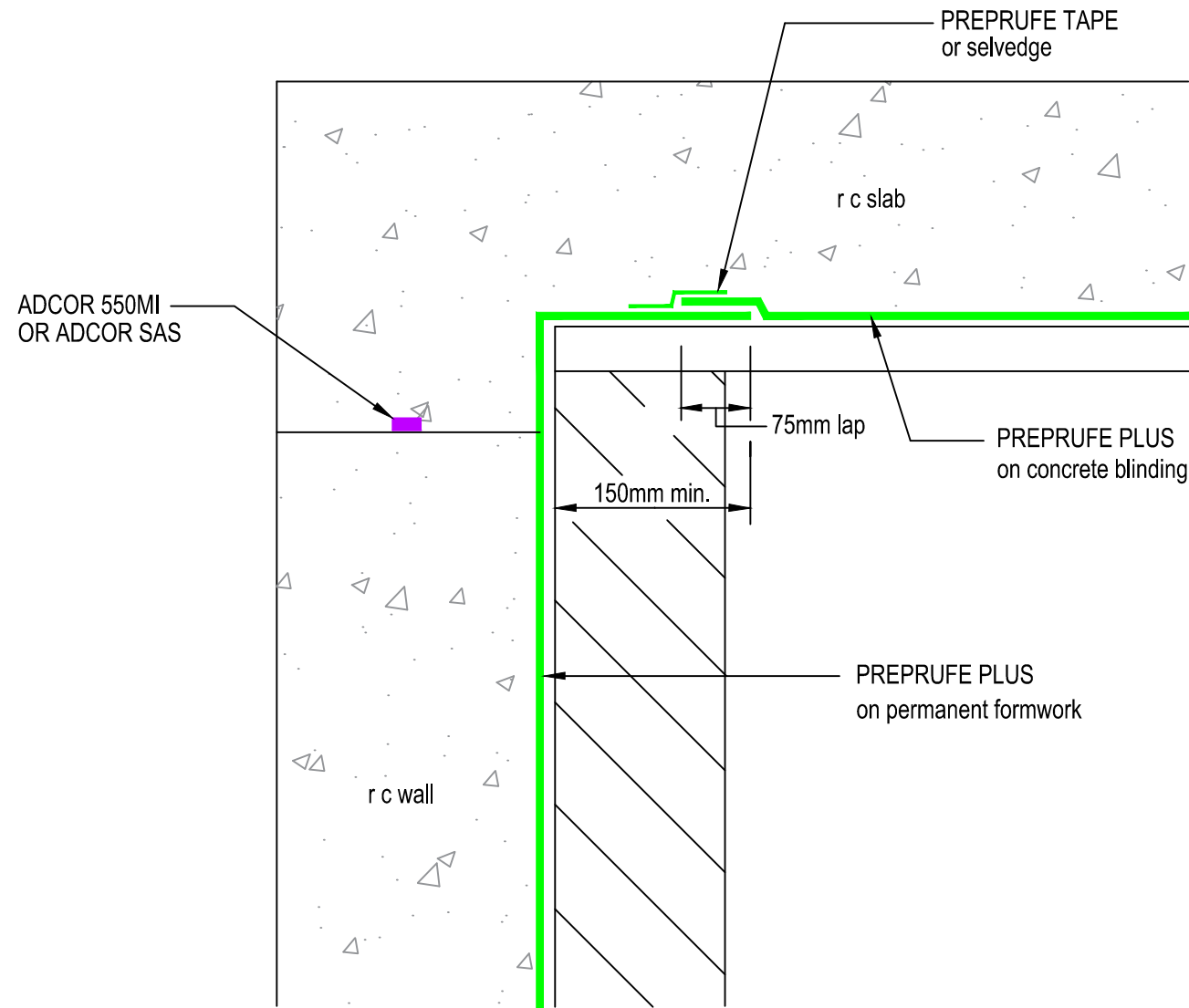
RC WALL TO UPPER LEVEL RC SLAB DETAIL SECTION
