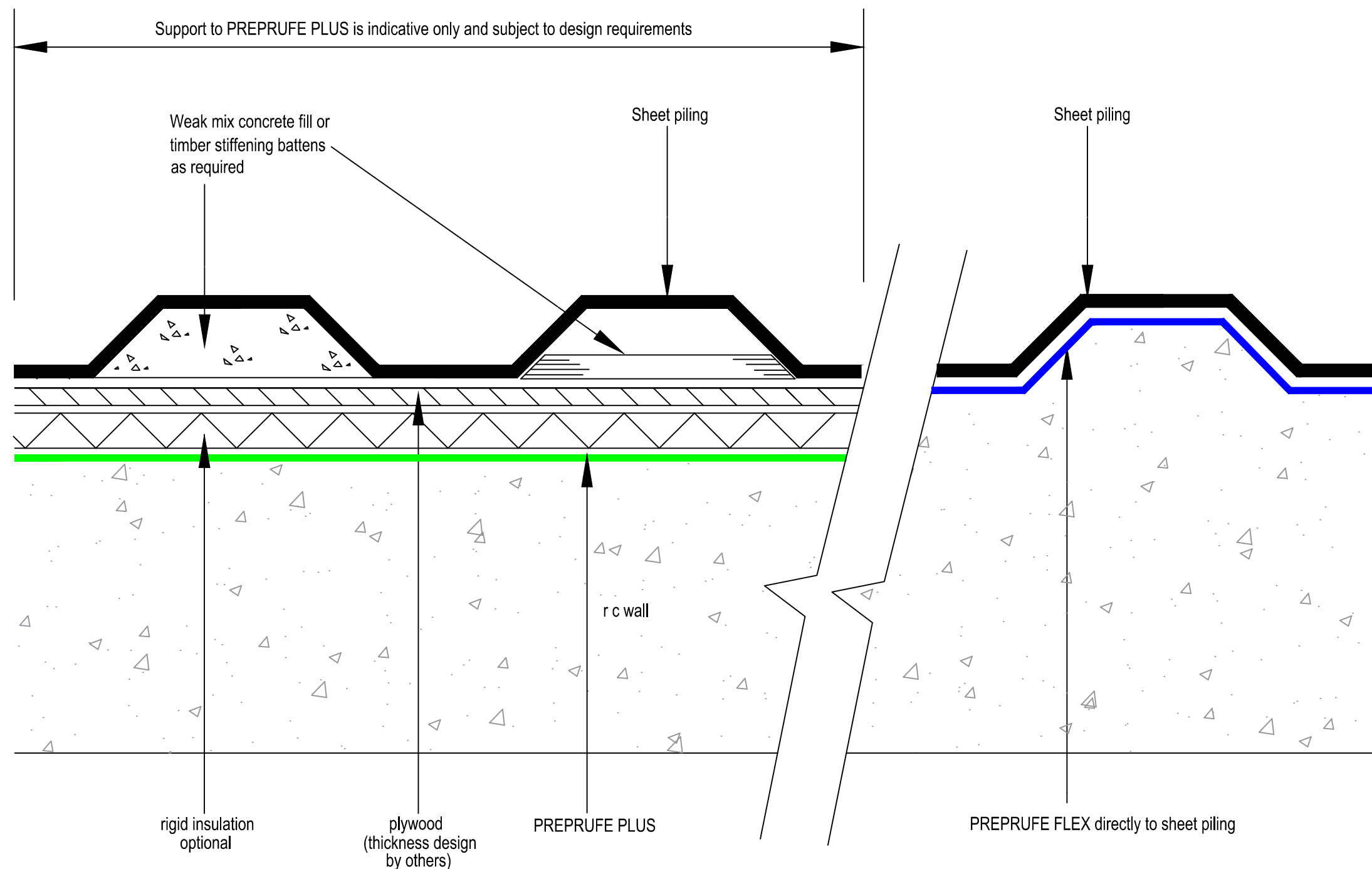
PREPRUFE PLUS ON FACED SHEET PILING PLAN
