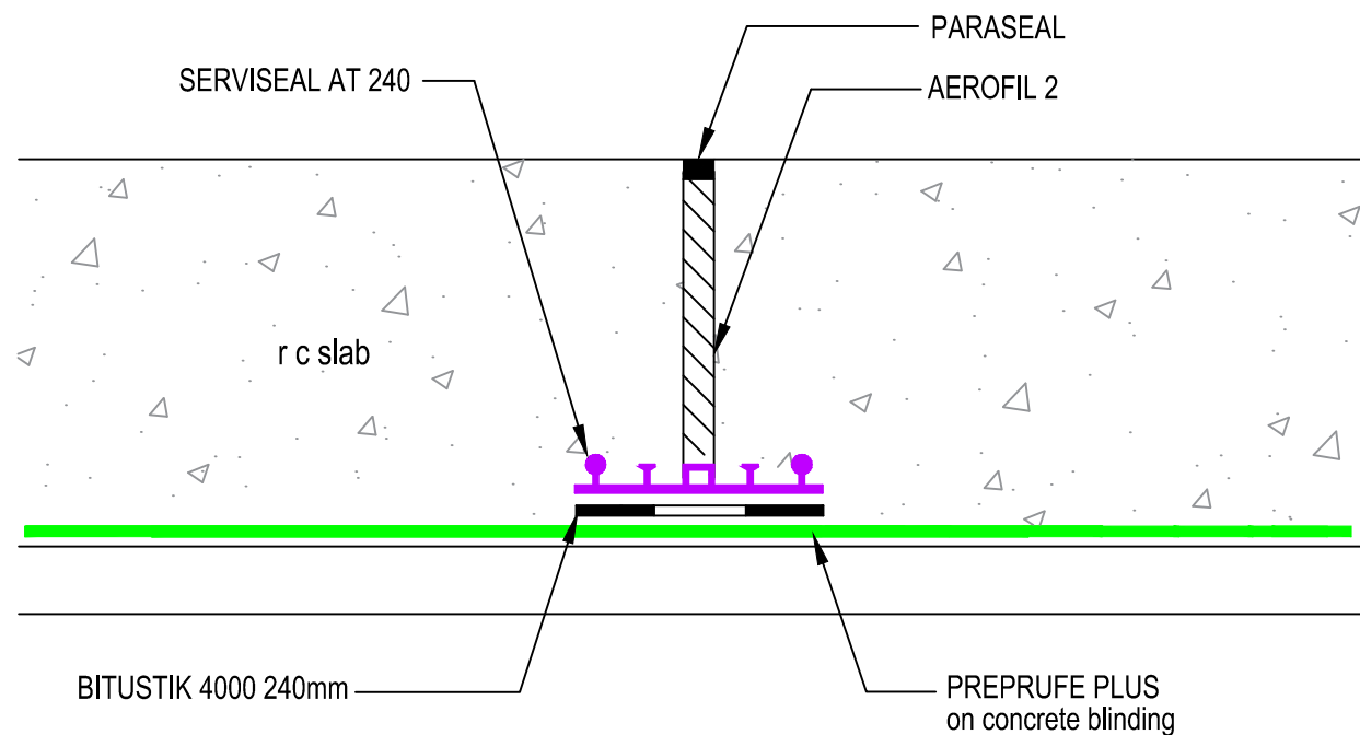
RC SLAB EXPANSION JOINT SECTION
