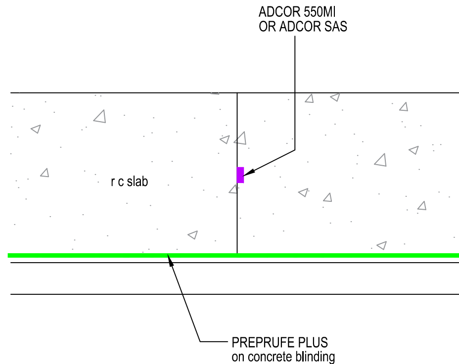
RC SLAB CONSTRUCTION JOINT SECTION
