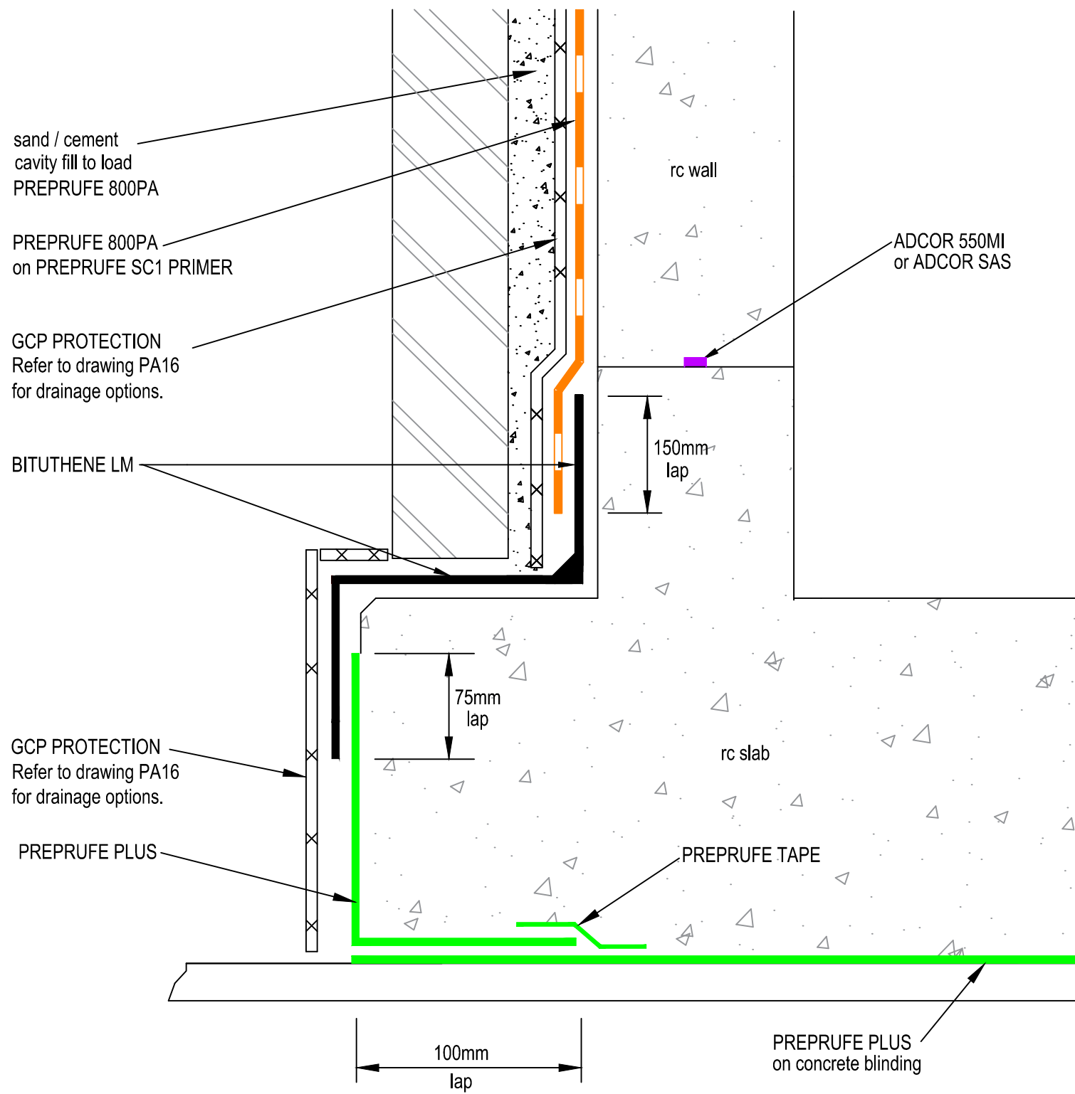
RC WALL BASE WITH TOE DETAIL SECTION
