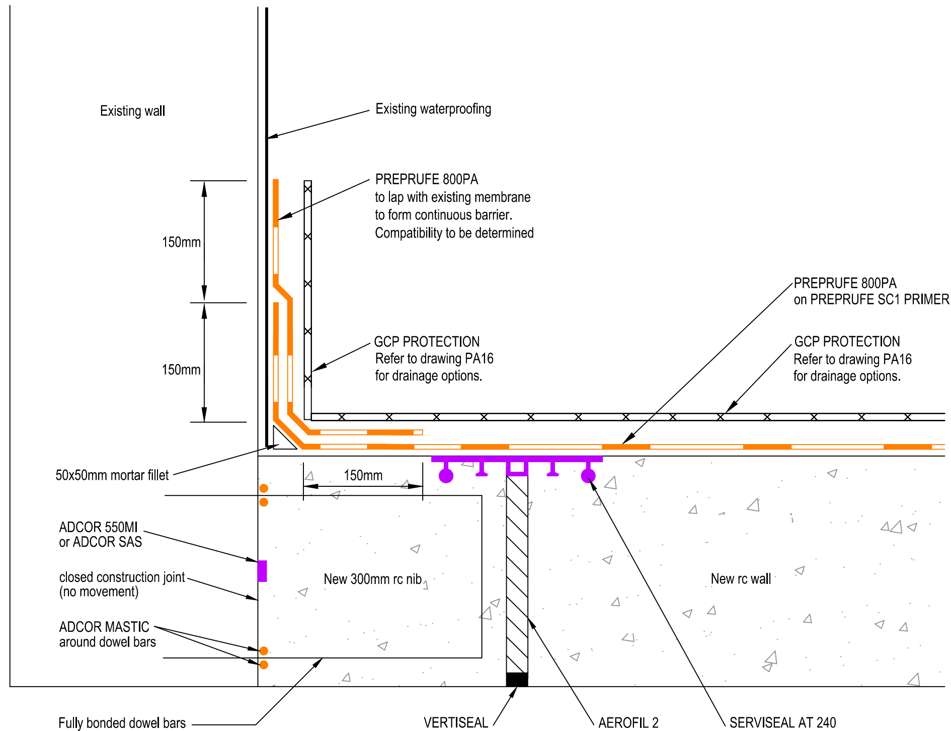
NEW TO EXISTING WALL DETAIL PLAN
