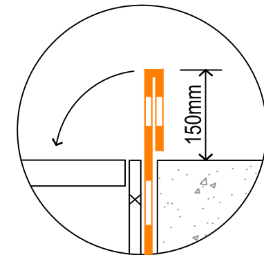
PREPRUFE 800PA bonded to itself to allow folding down to blinding
