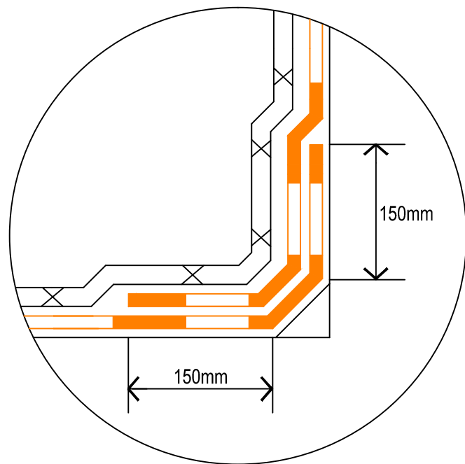
PREPRUFE 800PA CONFIGURATION HORIZONTAL TO VERTICAL
