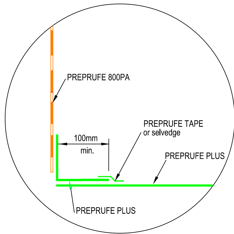
ALTERNATIVE PREPRUFE PLUS CONFIGURATION HORIZONTAL TO VERTICAL
