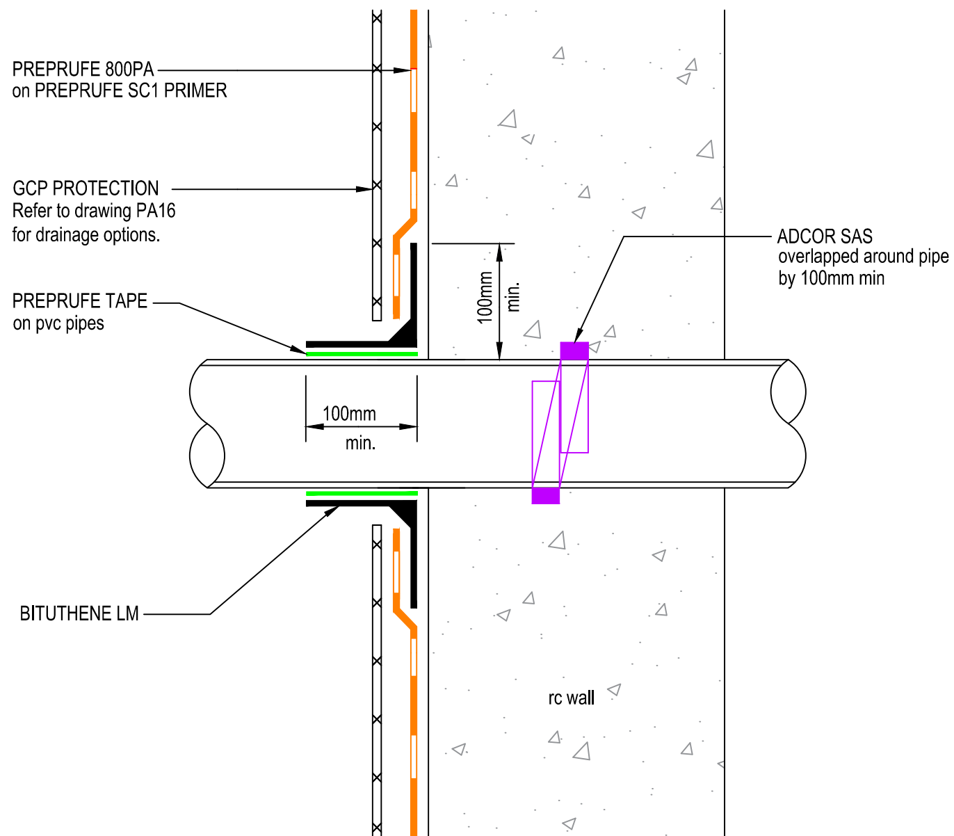
PIPE THROUGH RC WALL PLAN / SECTION
