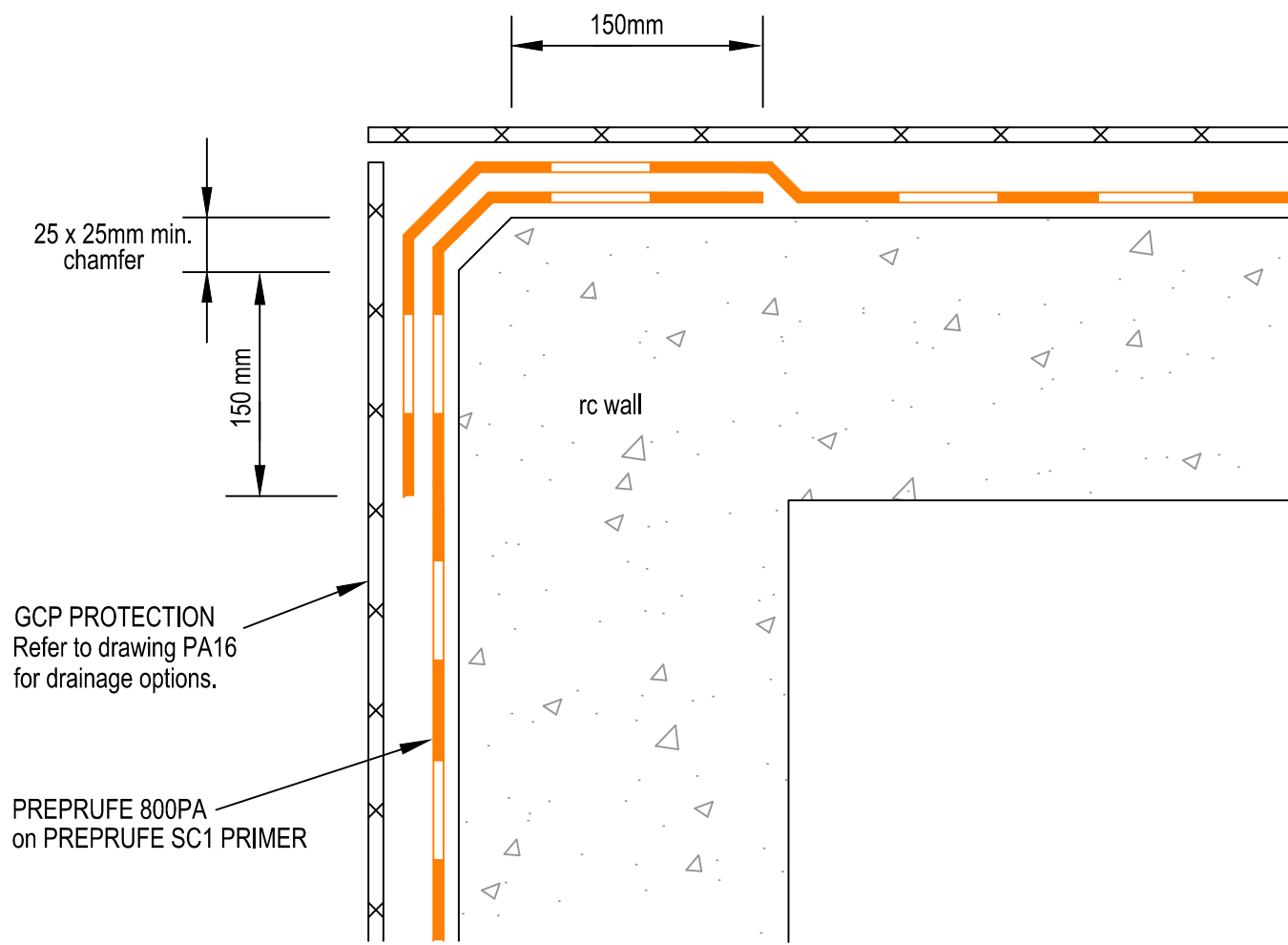
VERTICAL EXTERNAL CORNER PLAN
