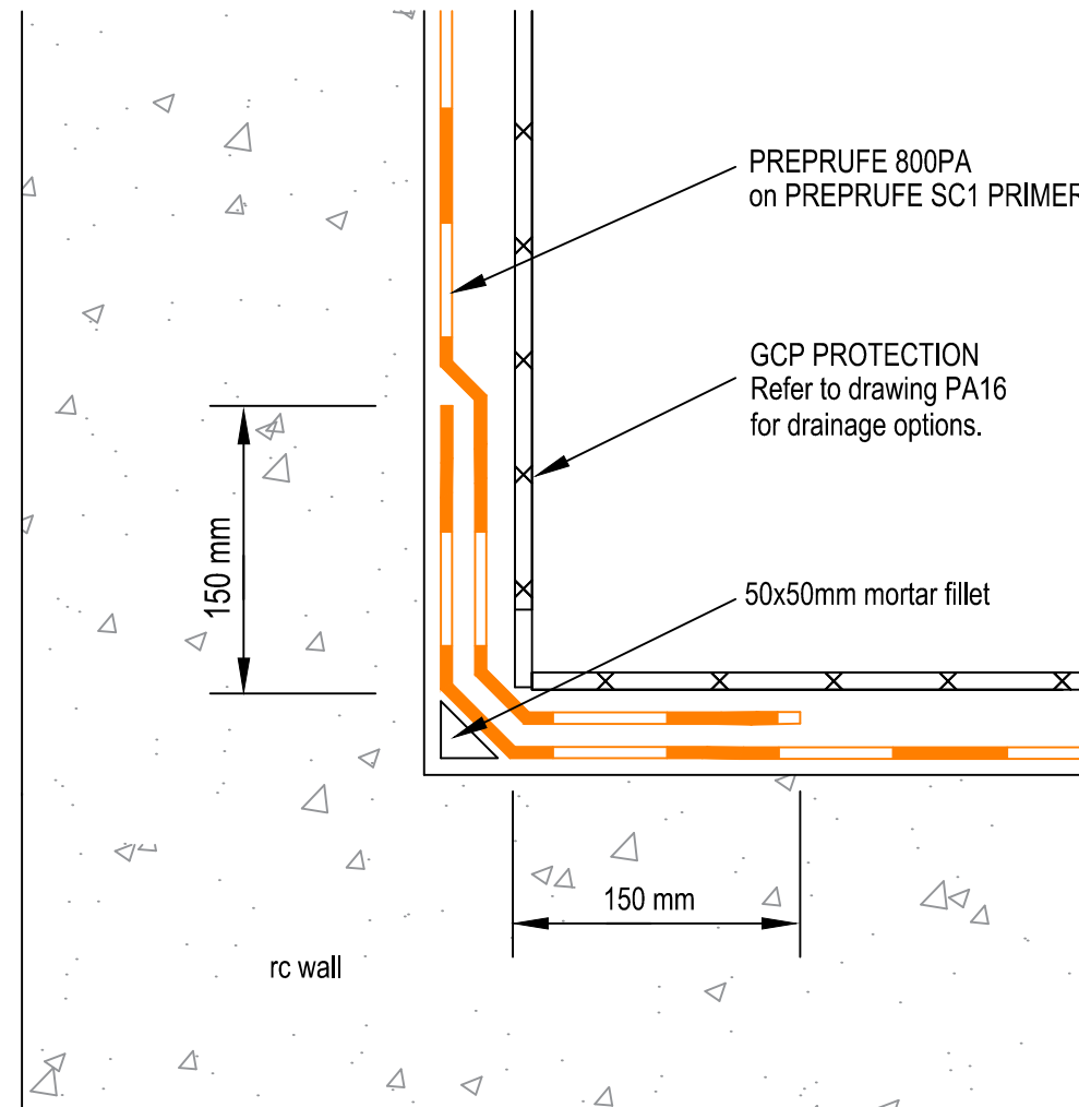
VERTICAL INTERNAL CORNER PLAN
