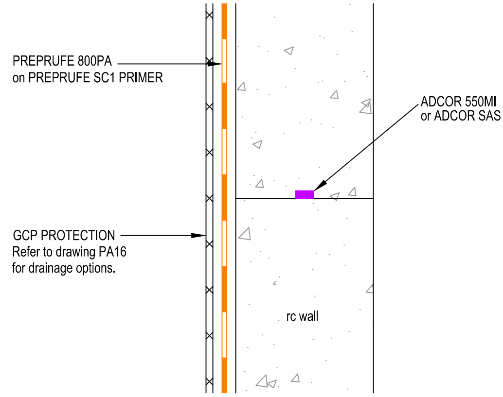
RC WALL CONSTRUCTION JOINT PLAN
