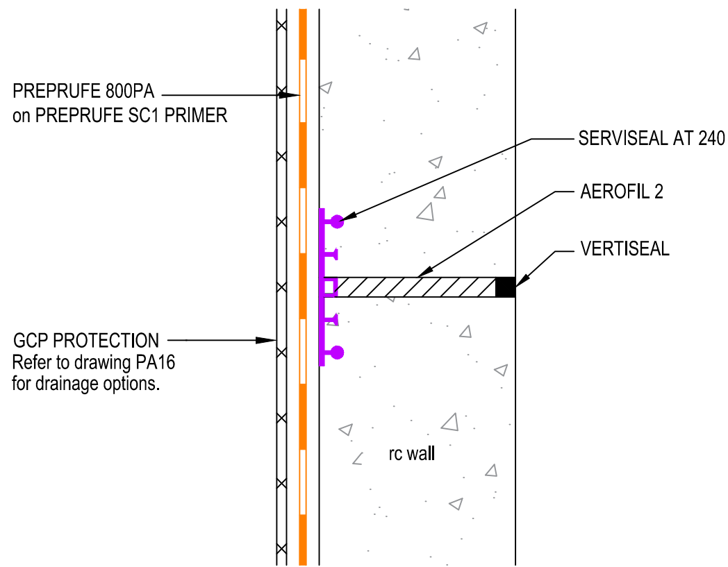
RC WALL EXPANSION JOINT PLAN
