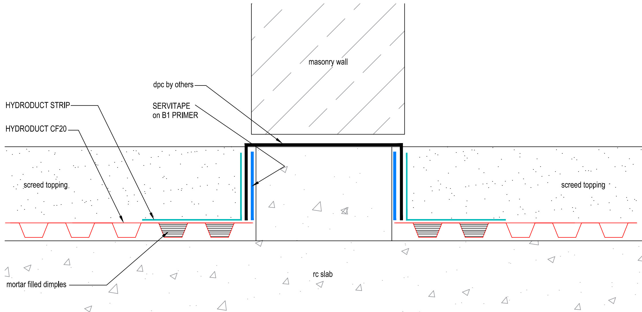
TERMINATION AT MASONRY DIVISION WALL SECTION
