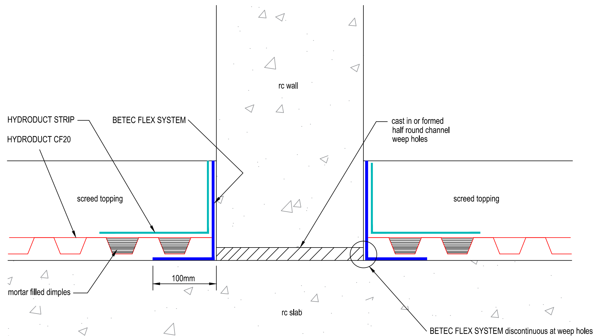
FLOW CONTINUITY THROUGH RC WALL SECTION
