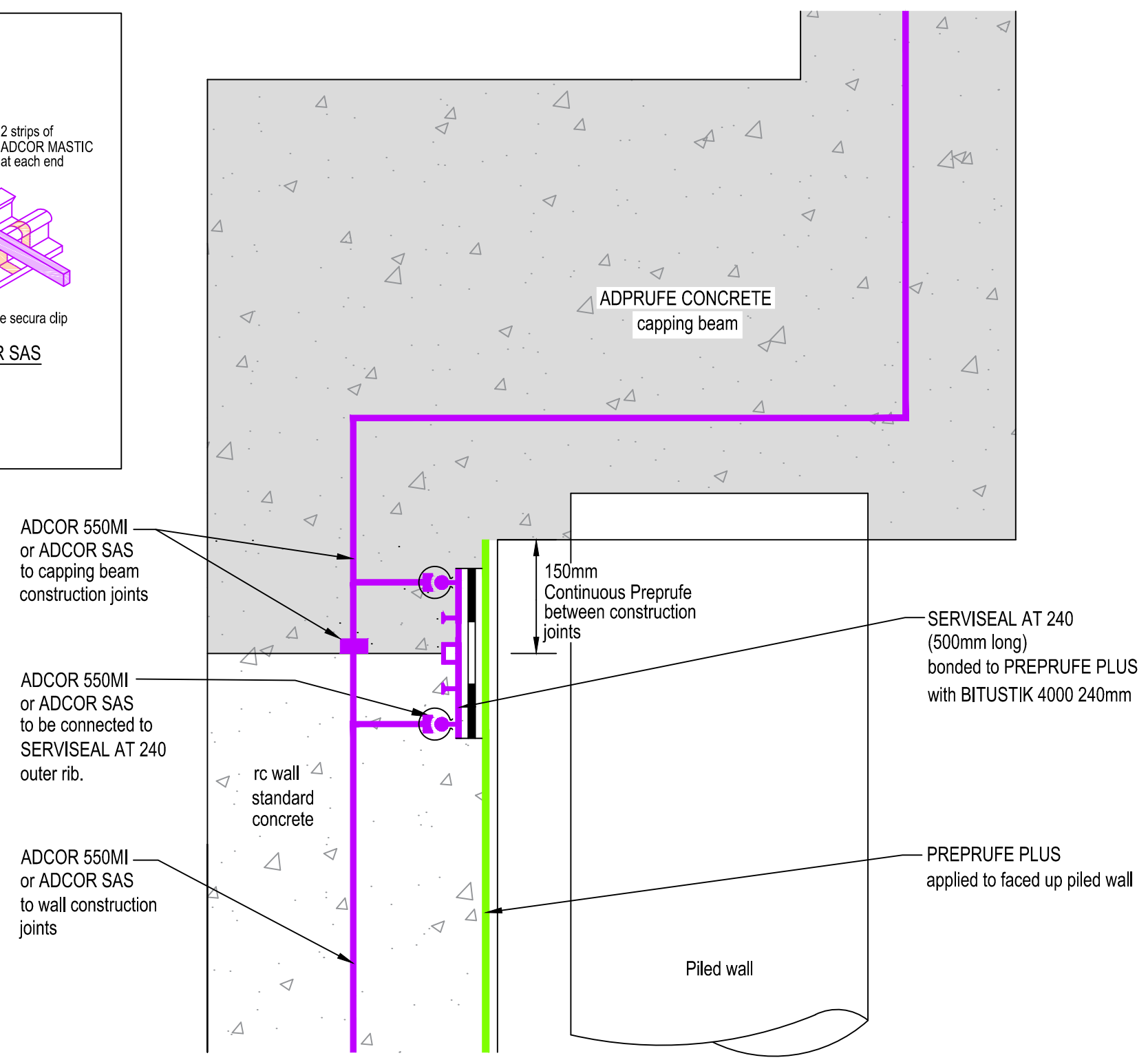
ADPRUFE / PREPRUFE PLUS INTERFACE DETAIL SECTION AT CONSTRUCTION JOINT
