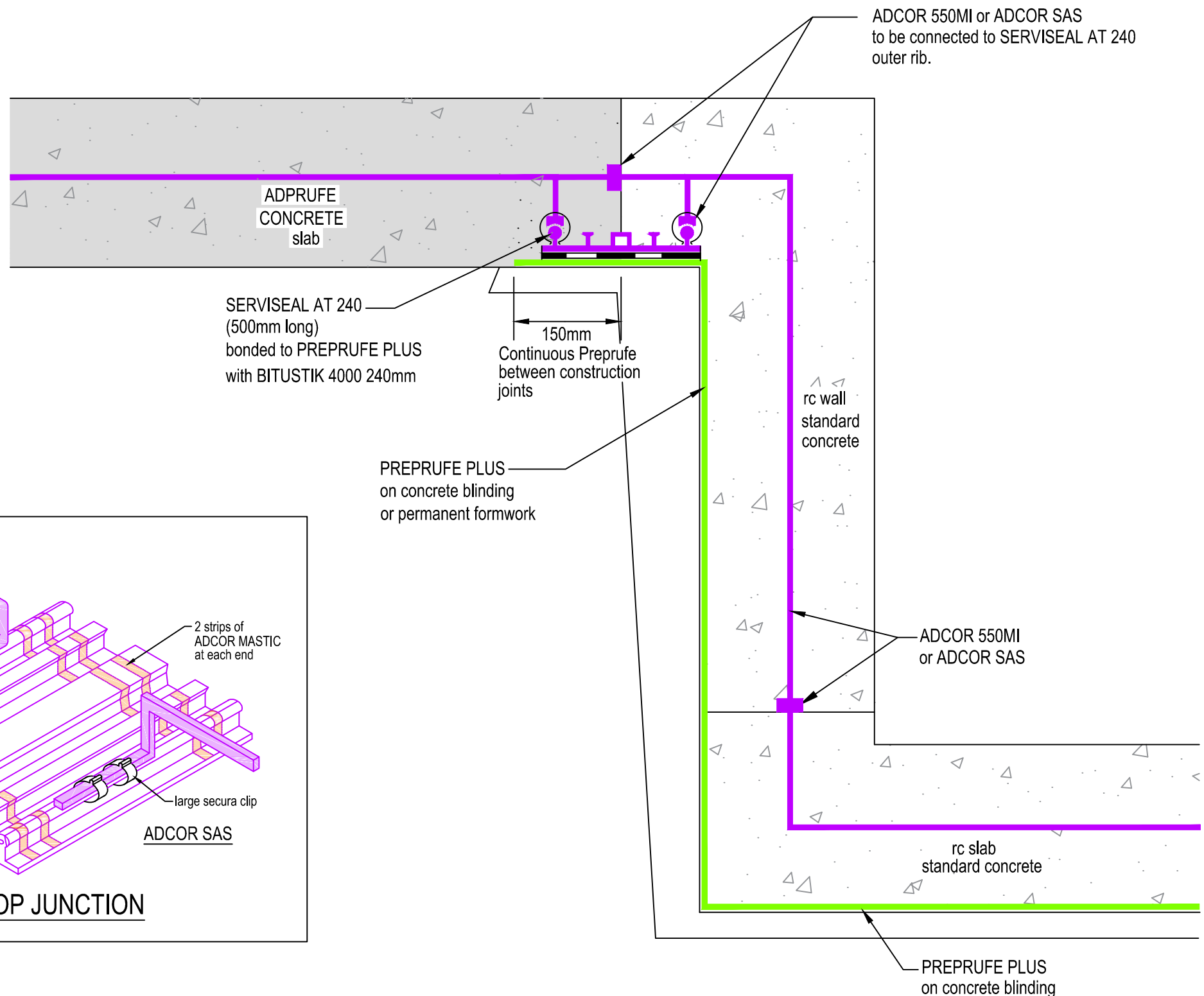
ADPRUFE / PREPRUFE PLUS INTERFACE DETAIL SECTION AT CONSTRUCTION JOINT
