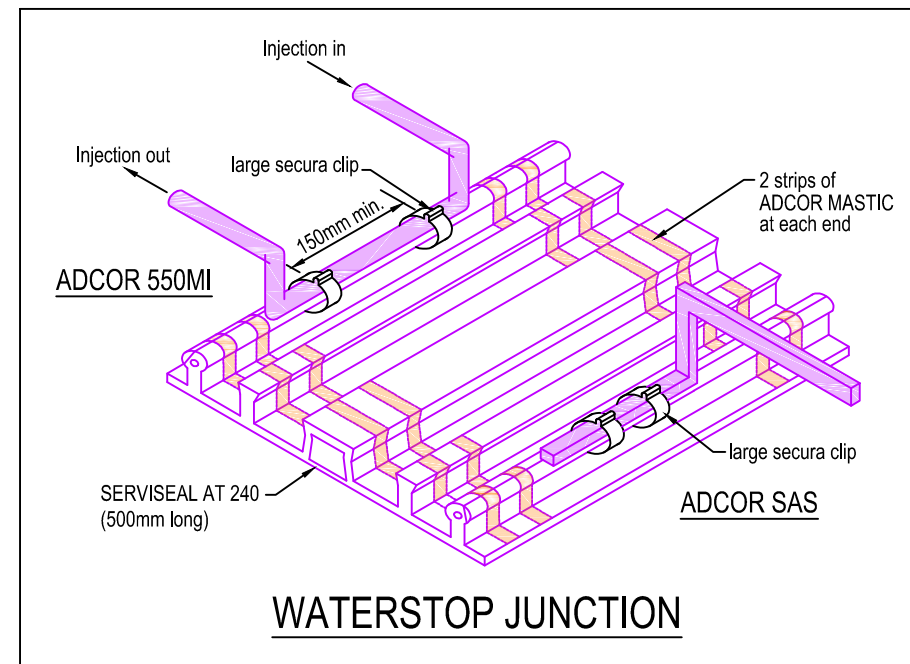
ADPRUFE / SERVIRUFE TRAFFIC DECK INTERFACE DETAIL SECTION AT CONSTRUCTION JOINT
