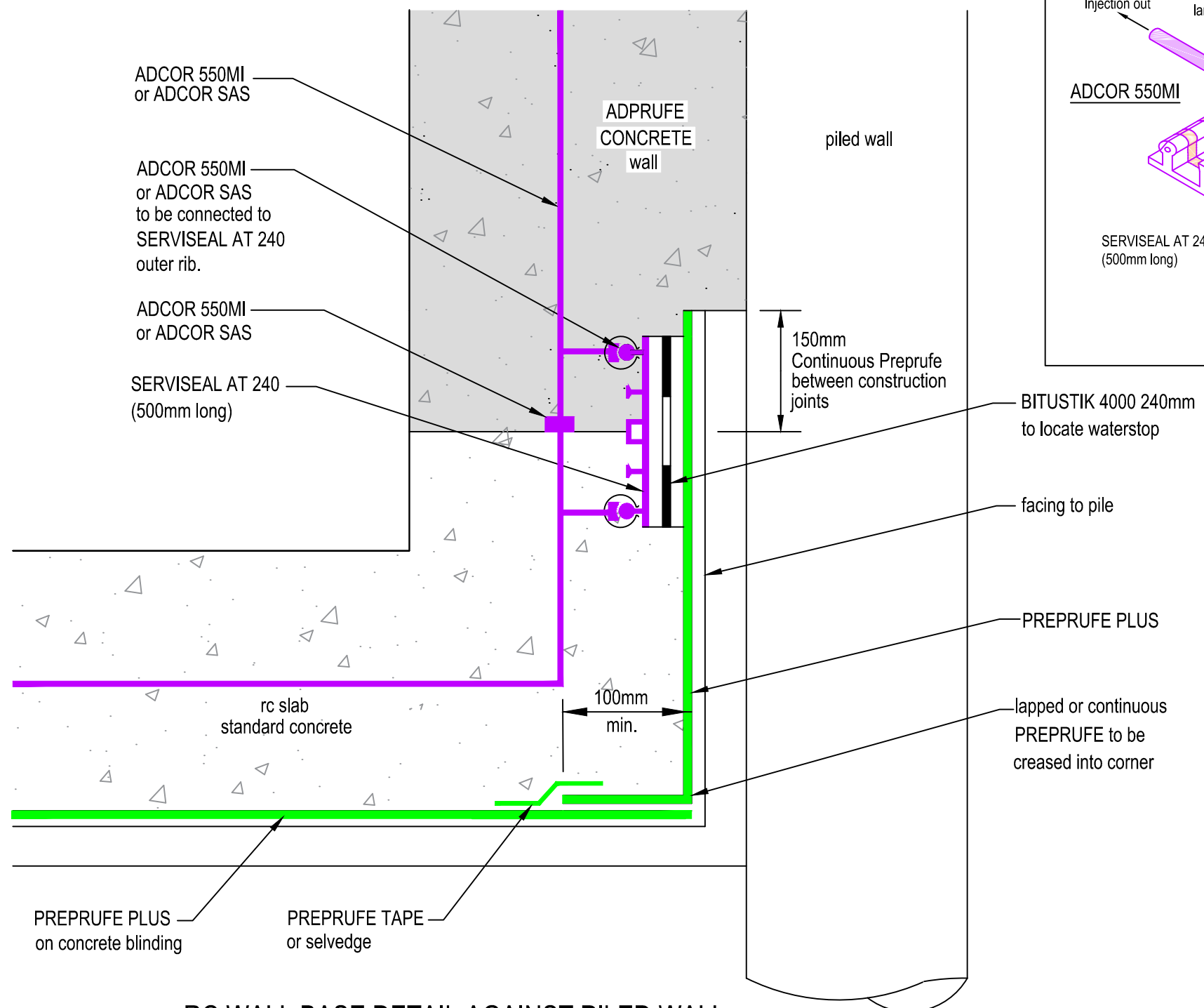
RC WALL BASE DETAIL AGAINST PILED WALL SECTION AT CONSTRUCTION JOINT
