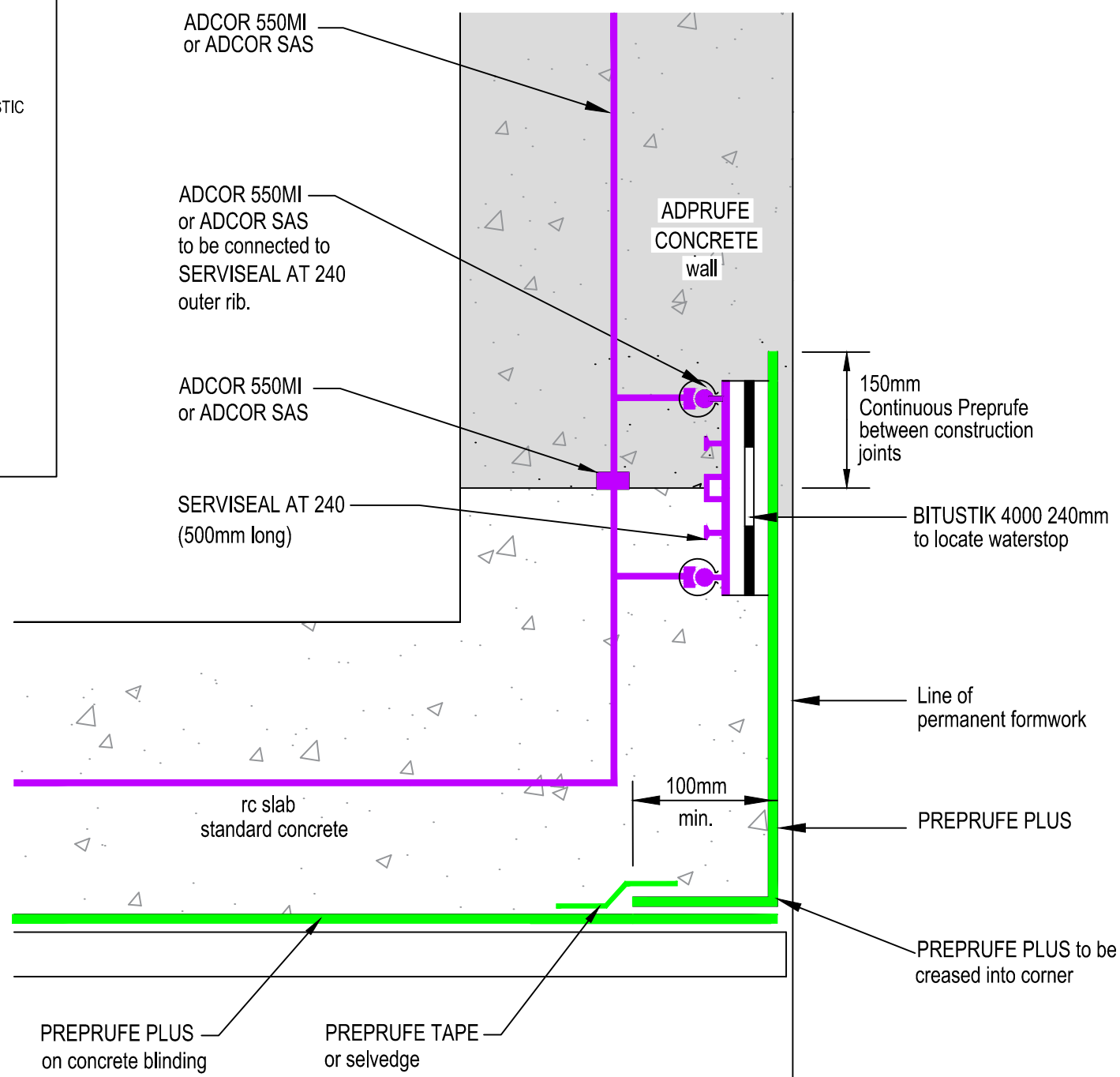
RC WALL BASE DETAIL AGAINST PERMANENT FORMWORK SECTION AT CONSTRUCTION JOINT
