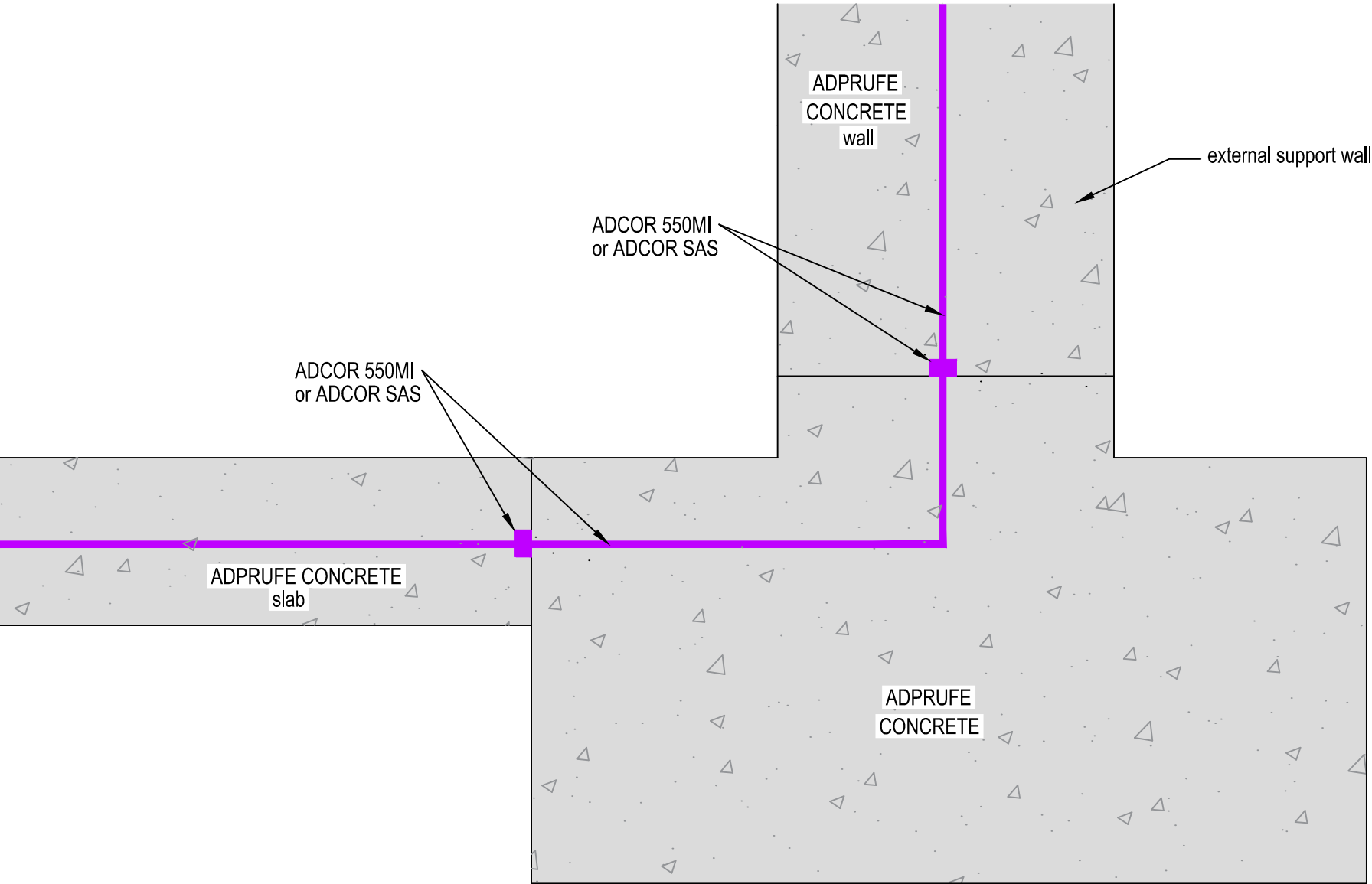
WALL BASE / SLAB JUNCTION SECTION AT CONSTRUCTION JOINTS
