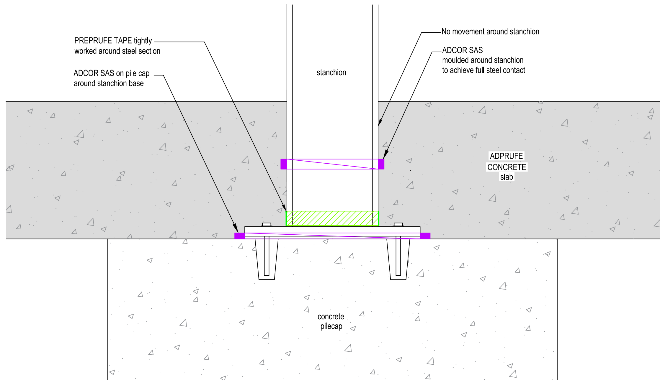
STANCHION THROUGH SLAB DETAIL SECTION
